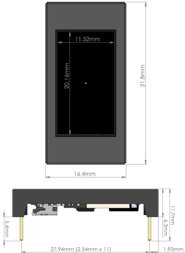
80x160 Pixel LCD Module ($89.99 incl SD Card)
